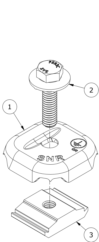
EXPLODED VIEW
