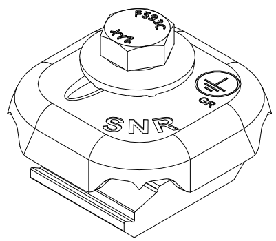
ASSEMBLED VIEW
