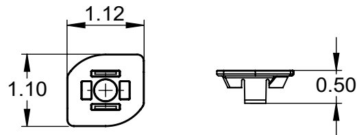
3) RETAINING CLIP
