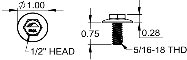
1) CAP SCREW, 5/16 X 3/4
